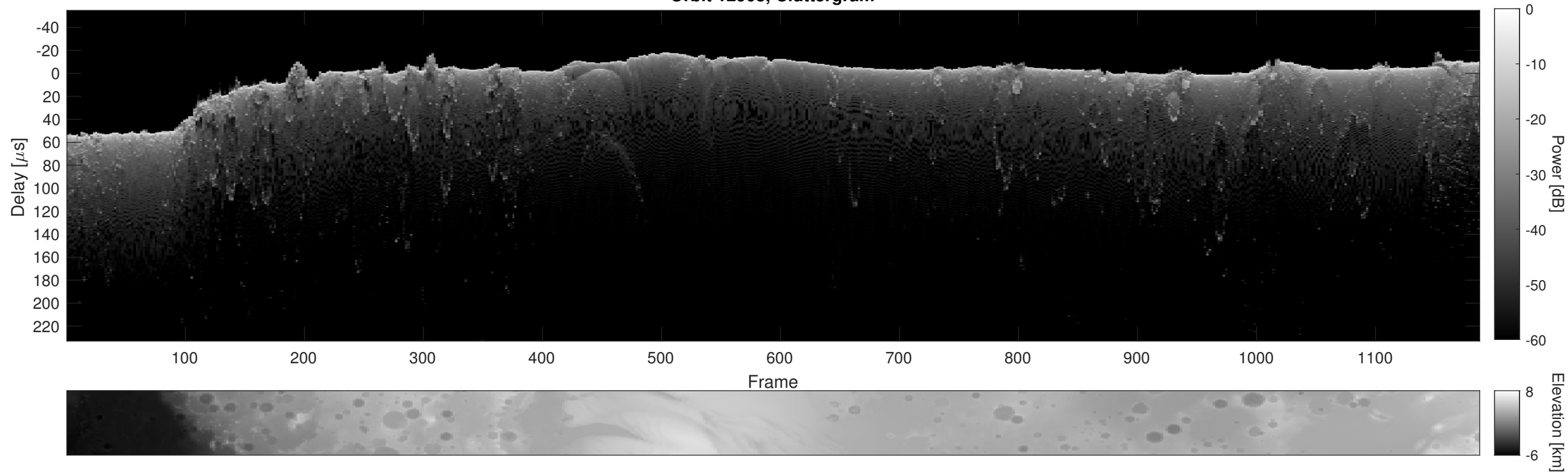
Orbit 12903, Cluttergram
