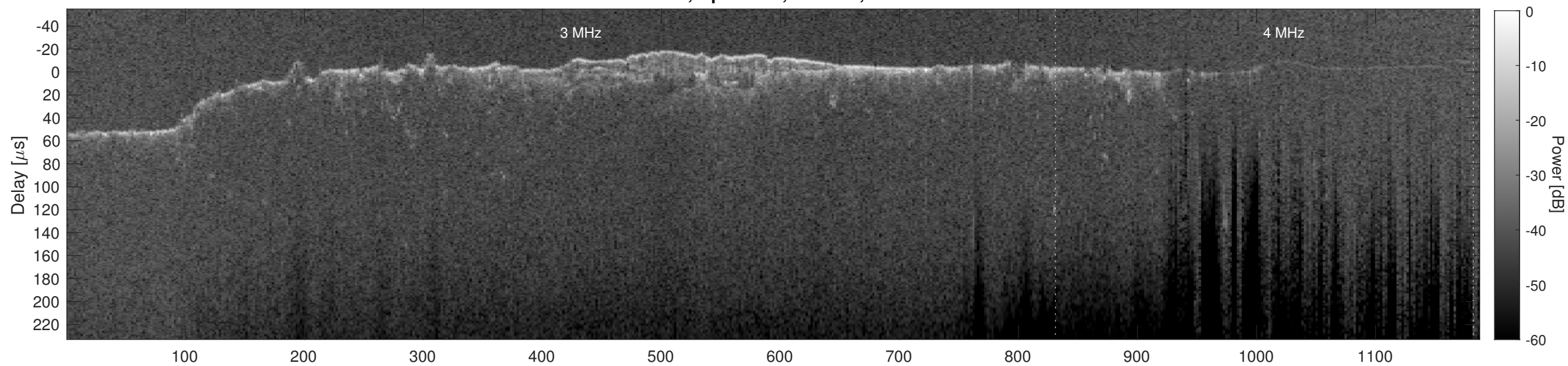
Orbit 12903, Cluttergram
