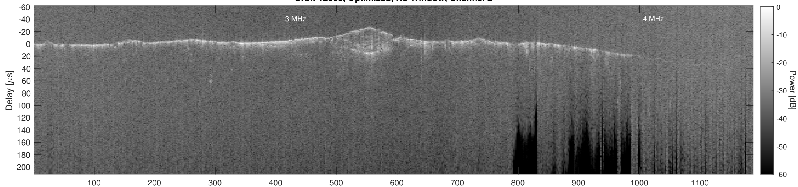
Orbit 12905, Cluttergram
