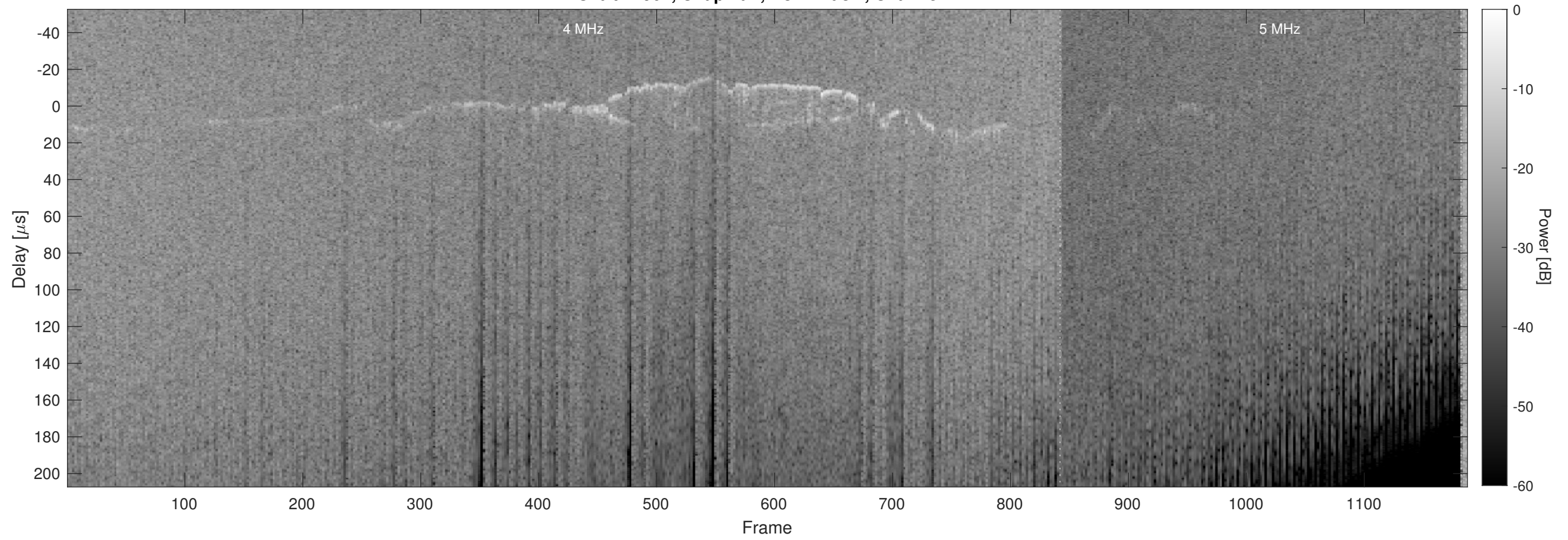
Orbit 12907, Chapman, No Window, Channel 2
