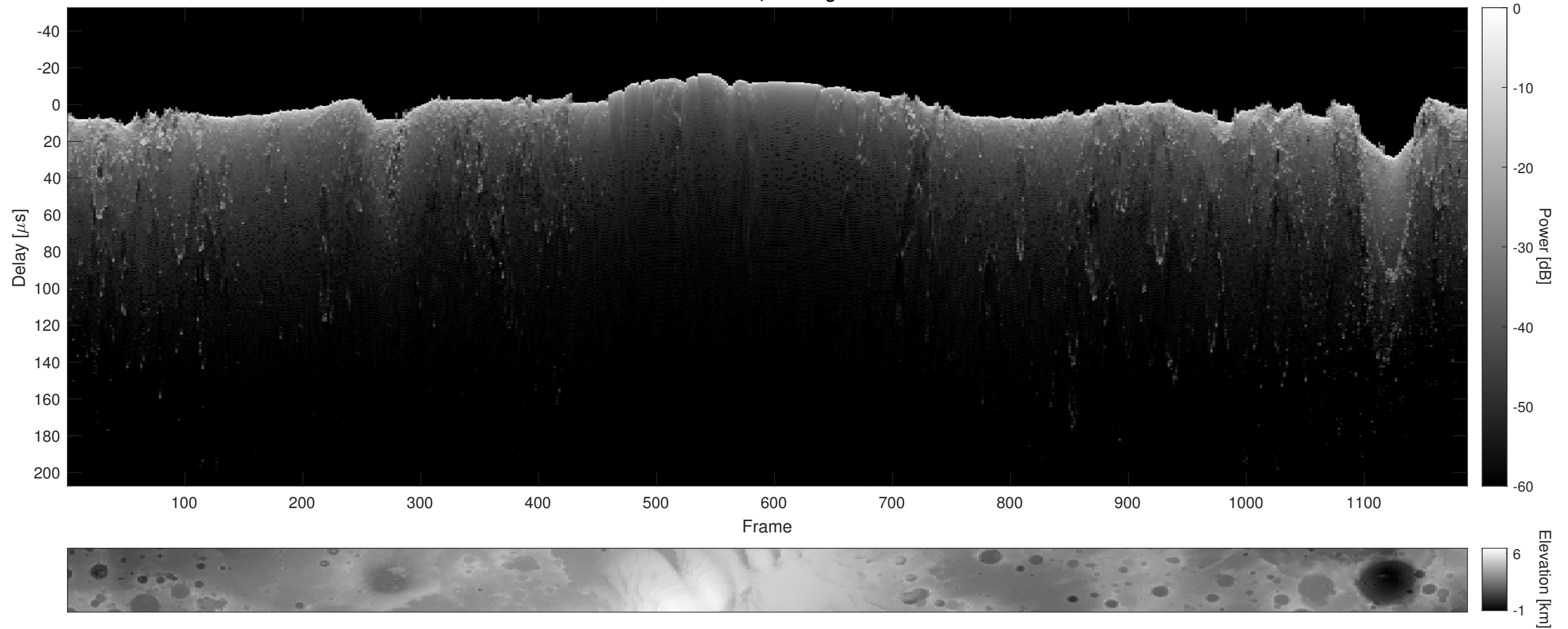
Orbit 12907, Cluttergram
