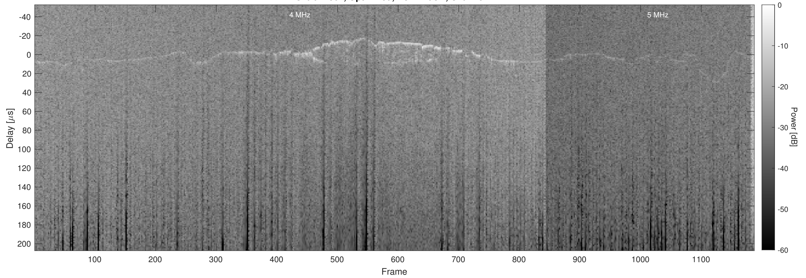
Orbit 12907, Optimized, No Window, Channel 2
