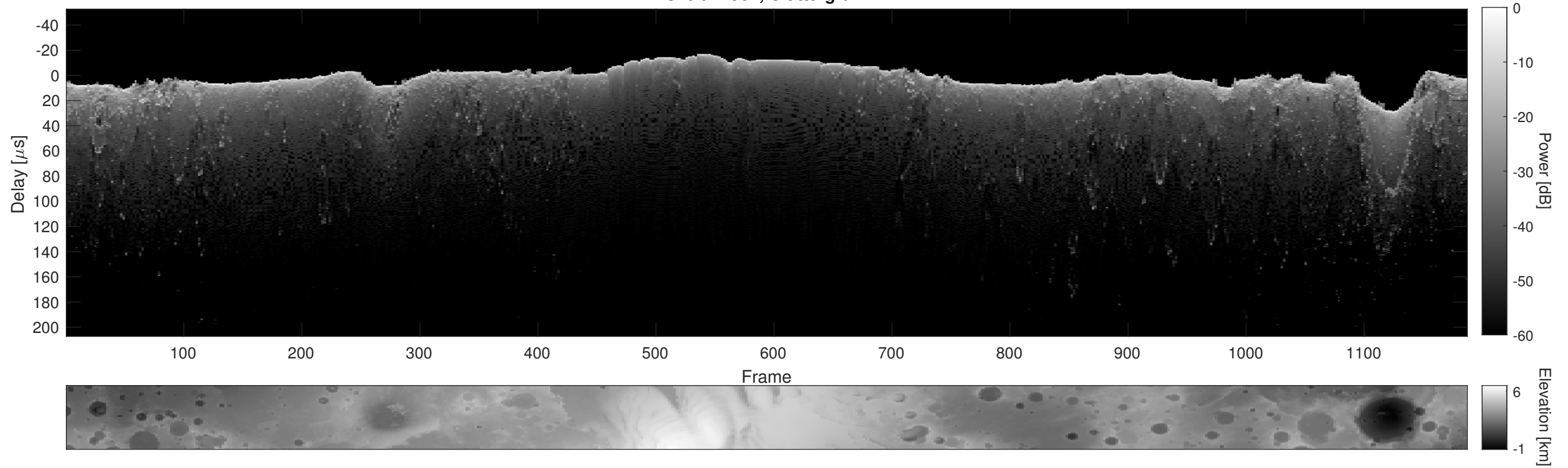
Orbit 12907, Cluttergram
