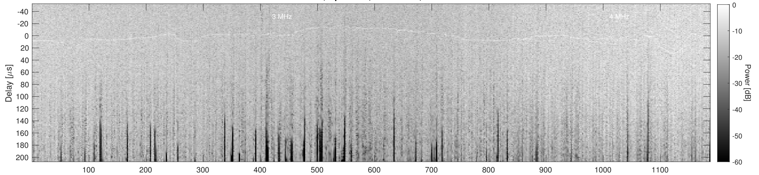
Orbit 12907, Cluttergram
