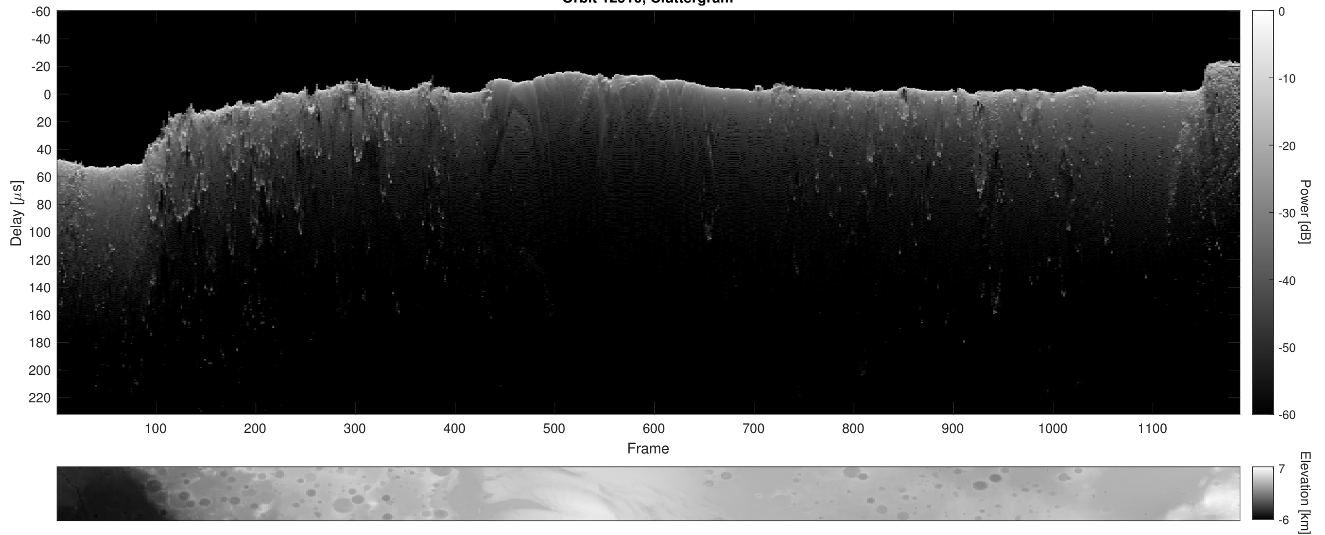
Orbit 12910, Cluttergram
