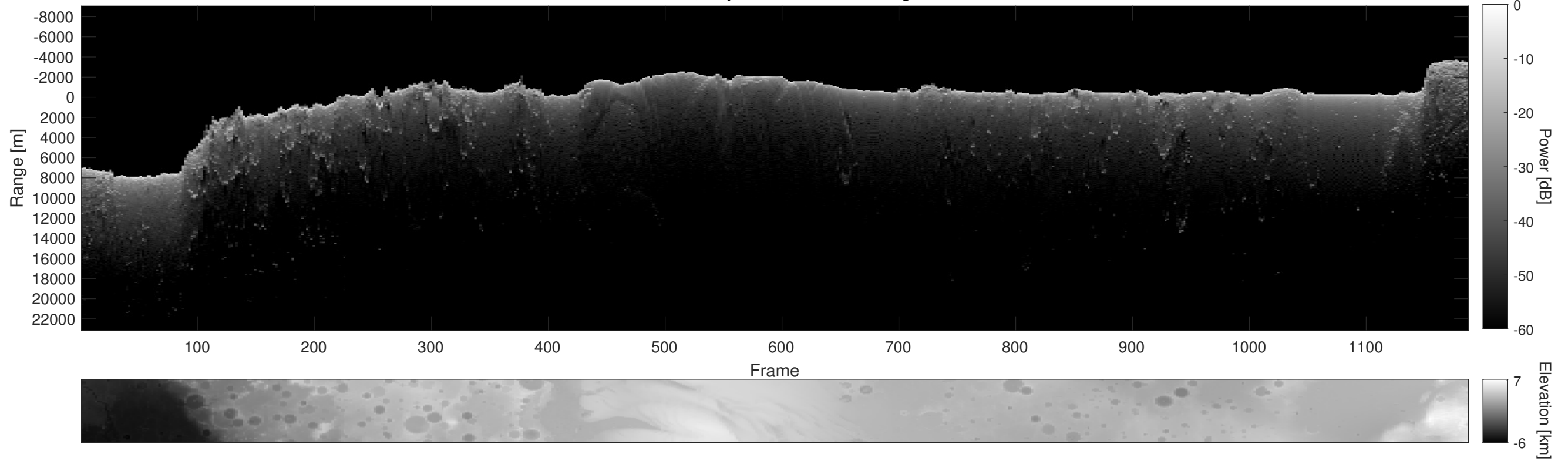
Orbit 12910, Depth-Corrected Cluttergram
