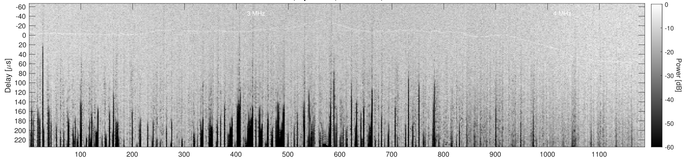
Orbit 12912, Cluttergram
