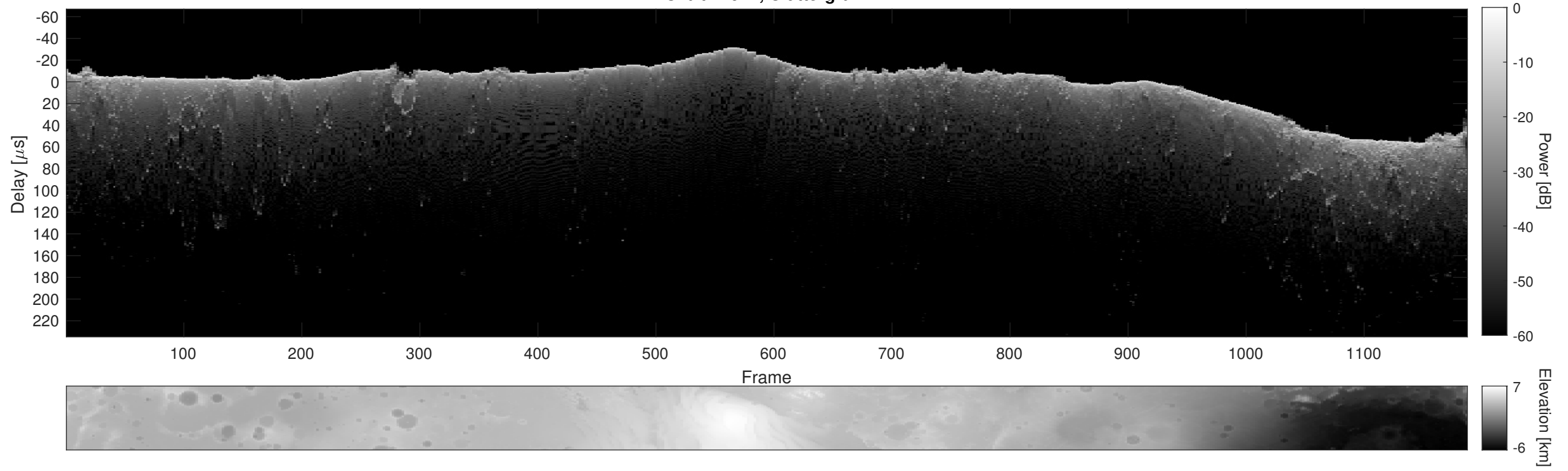
Orbit 12912, Cluttergram
