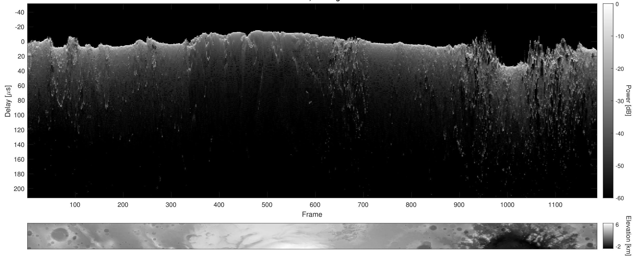
Orbit 12913, Cluttergram
