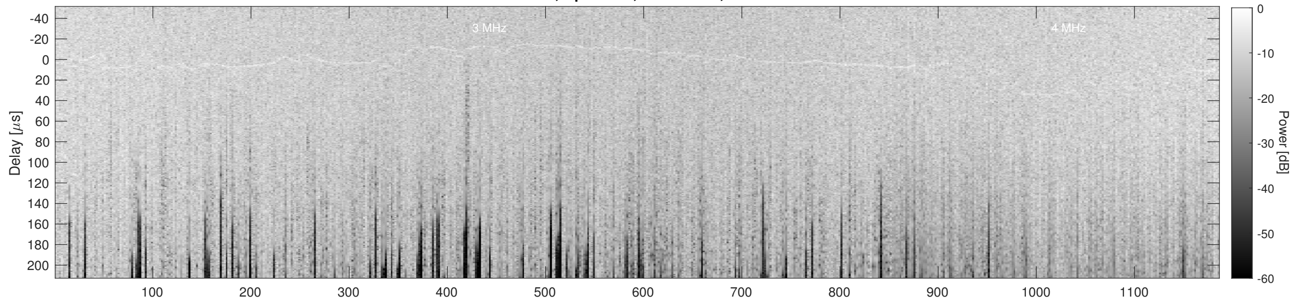
Orbit 12913, Cluttergram
