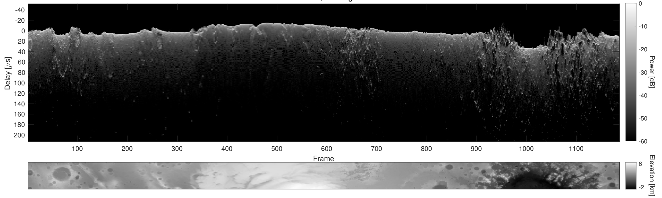
Orbit 12913, Cluttergram
