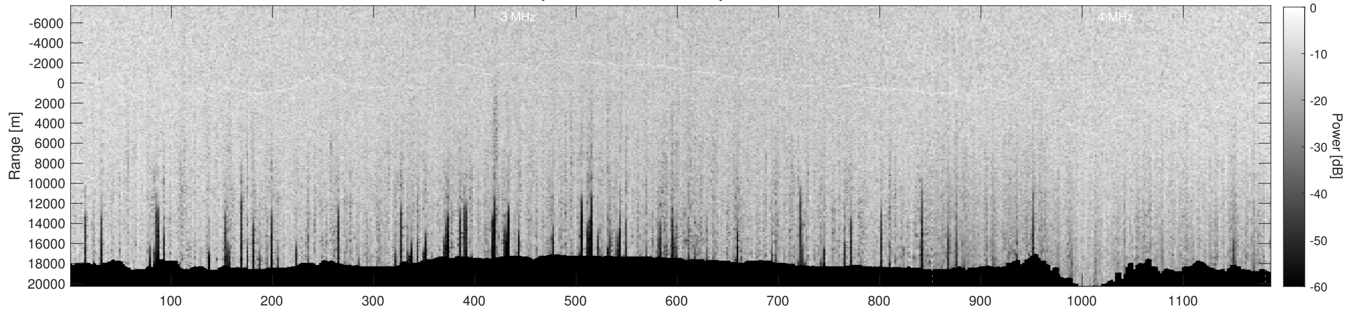
Orbit 12913, Depth-Corrected Cluttergram
