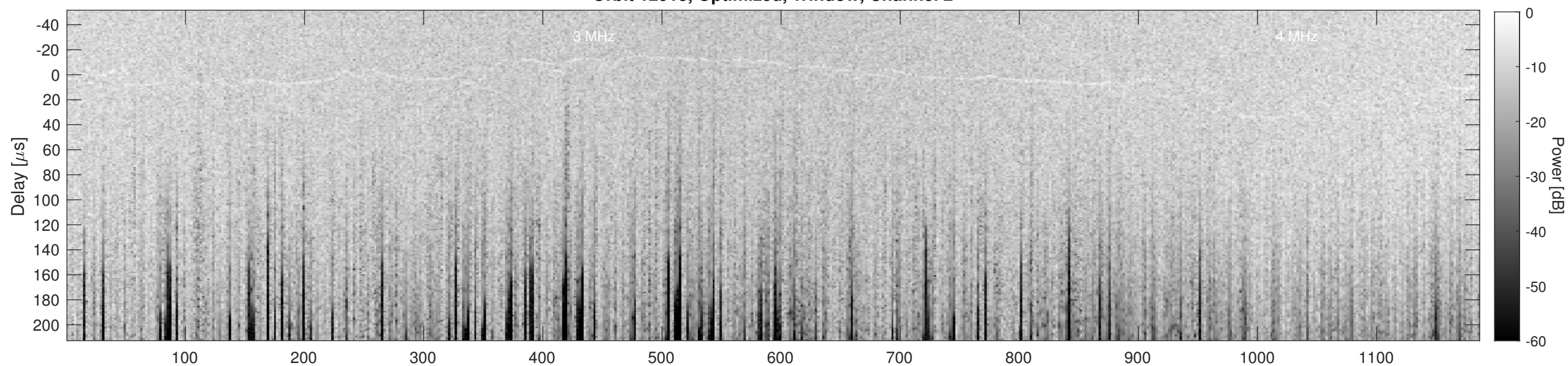
Orbit 12913, Cluttergram
