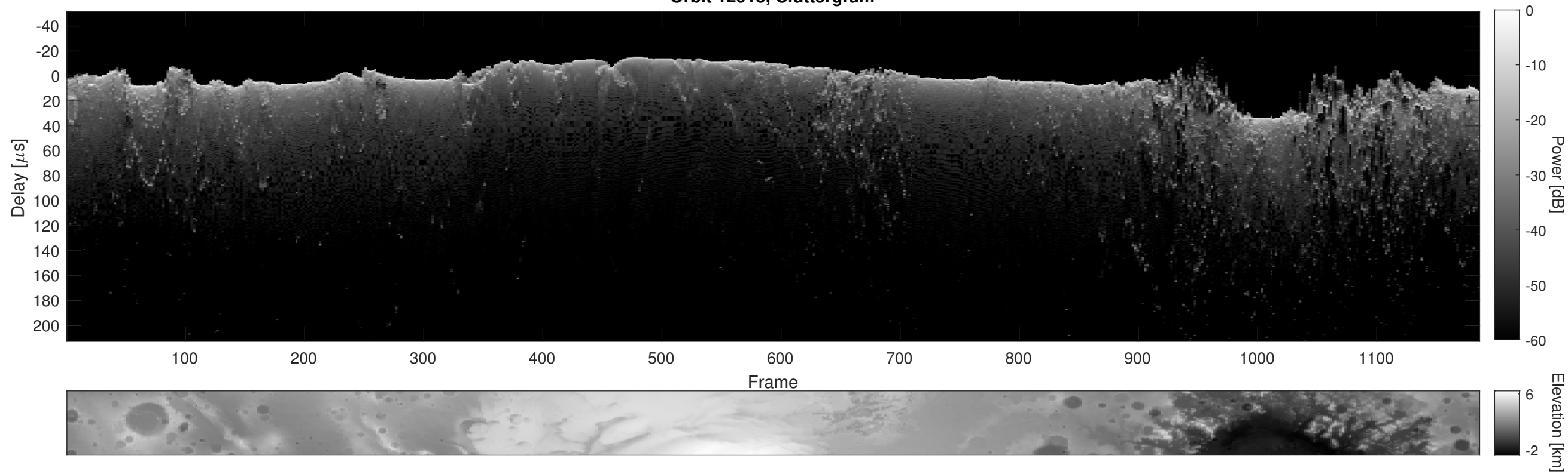
Orbit 12913, Cluttergram
