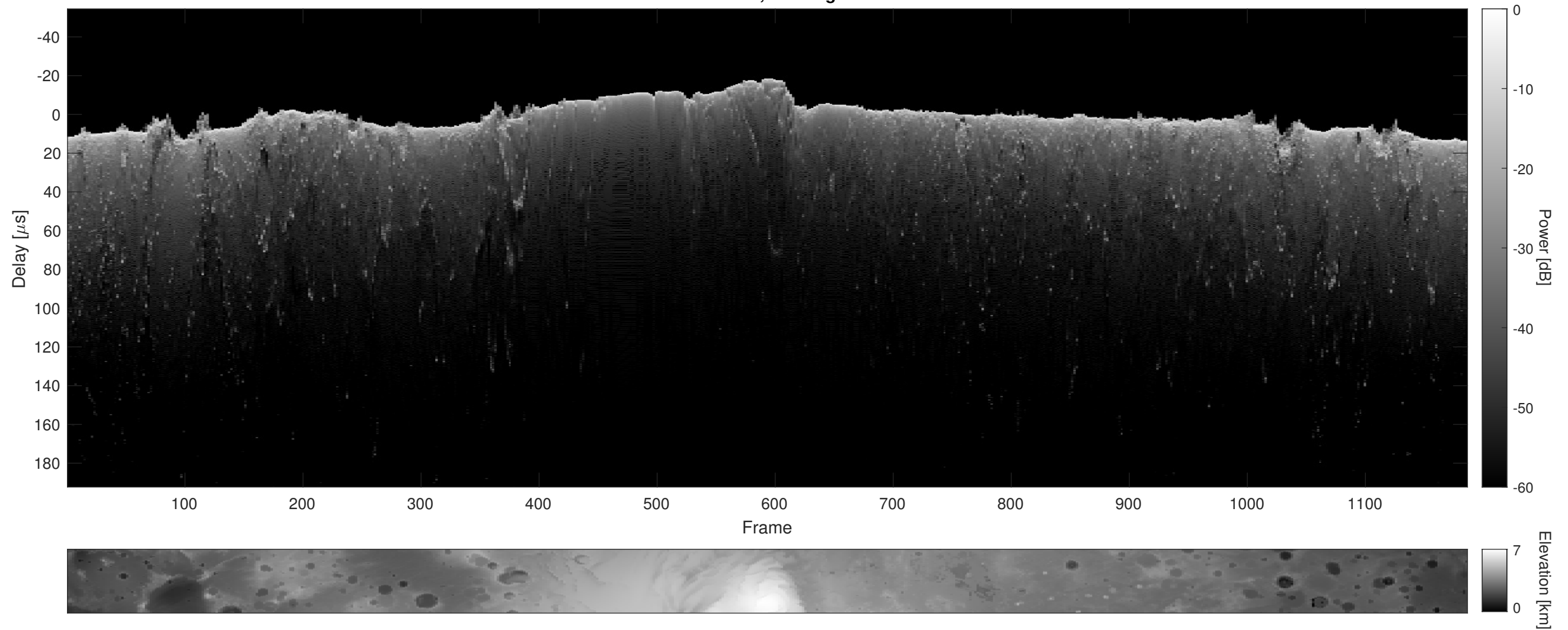
Orbit 12916, Cluttergram
