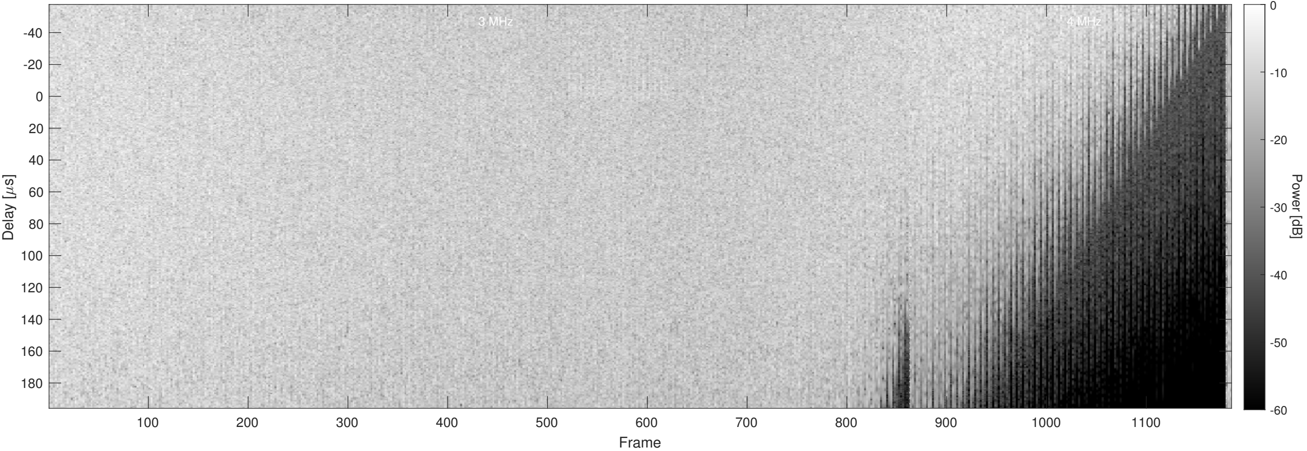
Orbit 12922, Chapman, No Window, Channel 2
