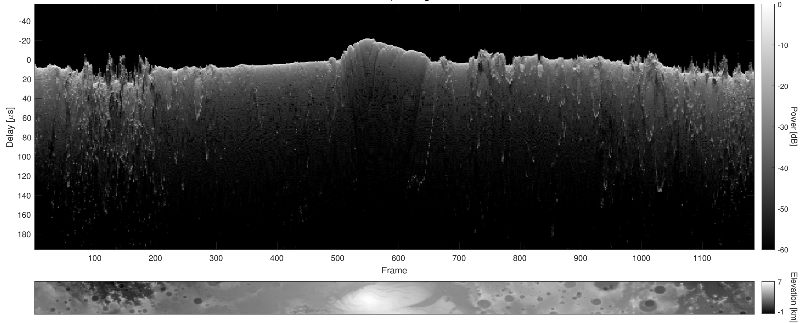
Orbit 12922, Cluttergram
