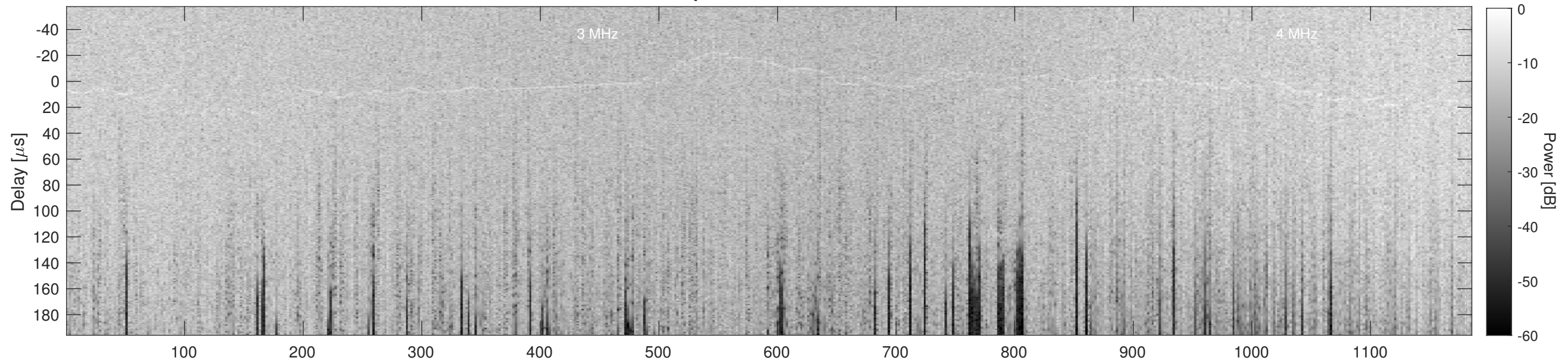
Orbit 12922, Cluttergram
