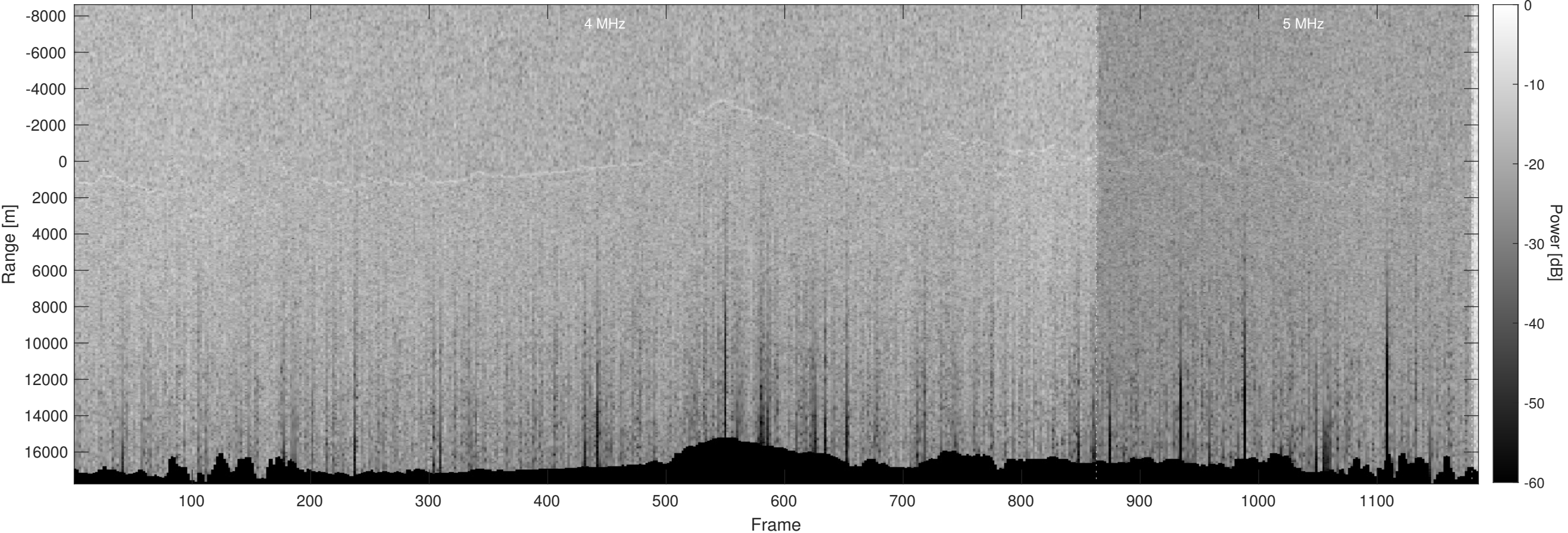
Orbit 12922, Optimized, No Window, Depth-Corrected, Channel 2
