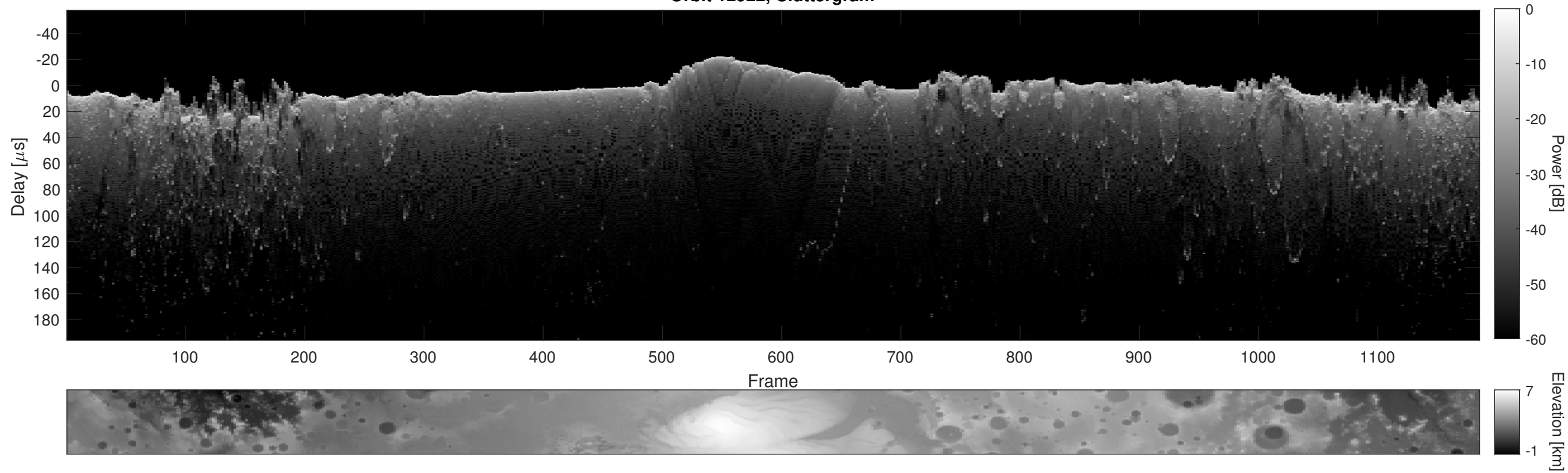
Orbit 12922, Cluttergram
