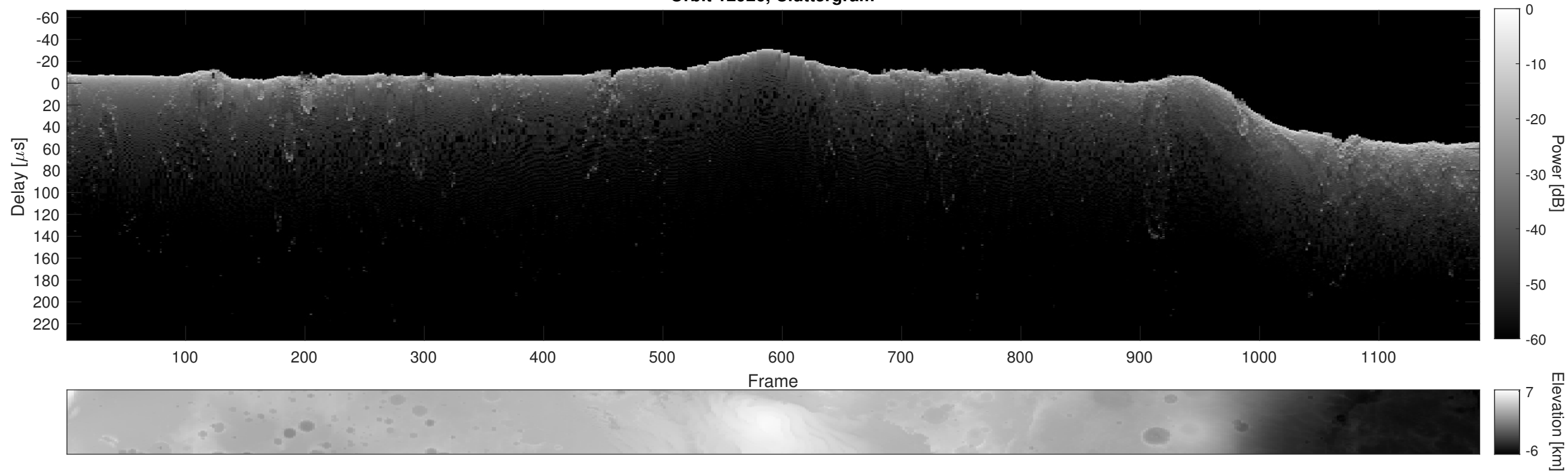
Orbit 12926, Cluttergram
