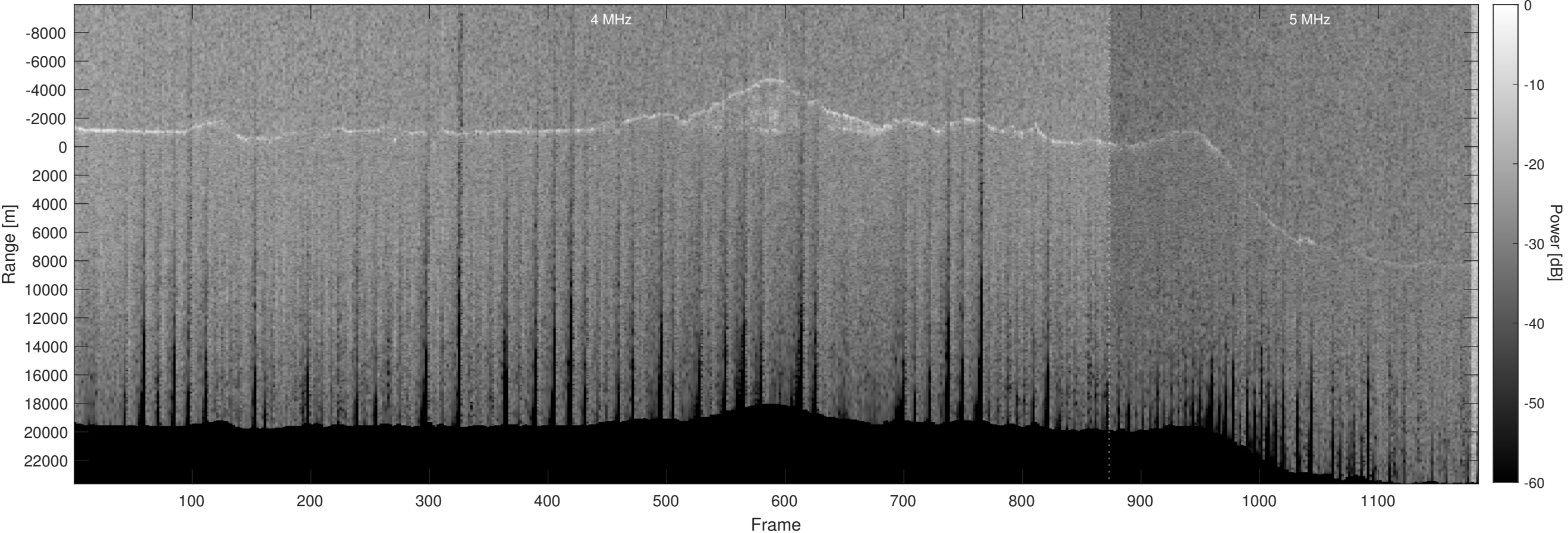
Orbit 12926, Optimized, No Window, Depth-Corrected, Channel 2
