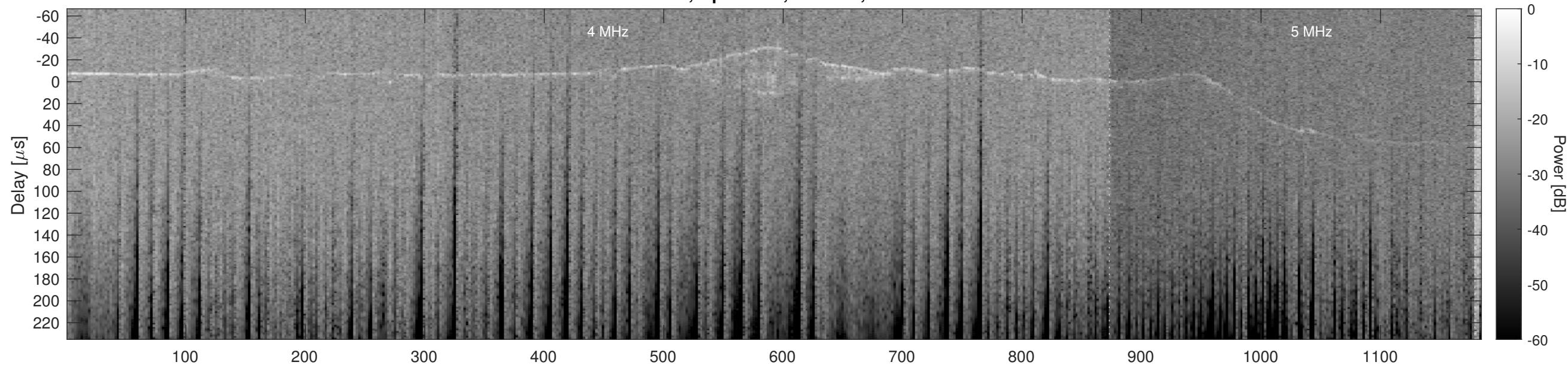
Orbit 12926, Optimized, Window, Channel 2
