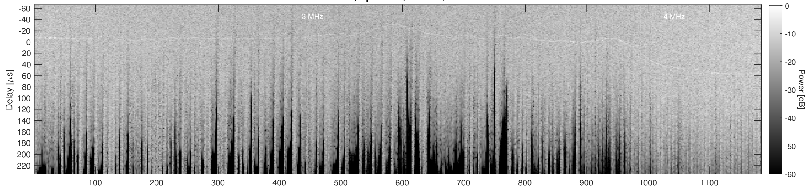
Orbit 12926, Cluttergram
