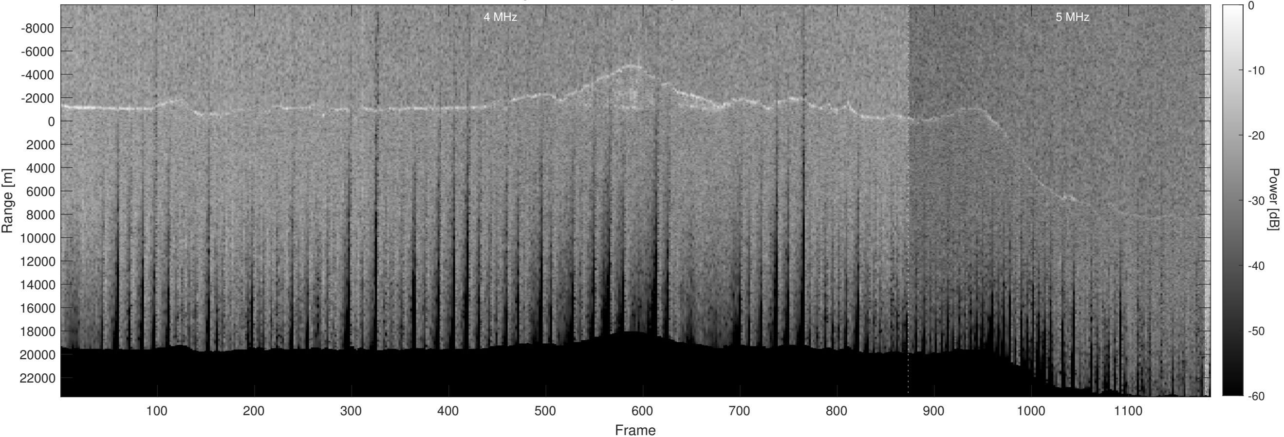
Orbit 12926, Optimized, Window, Depth-Corrected, Channel 2
