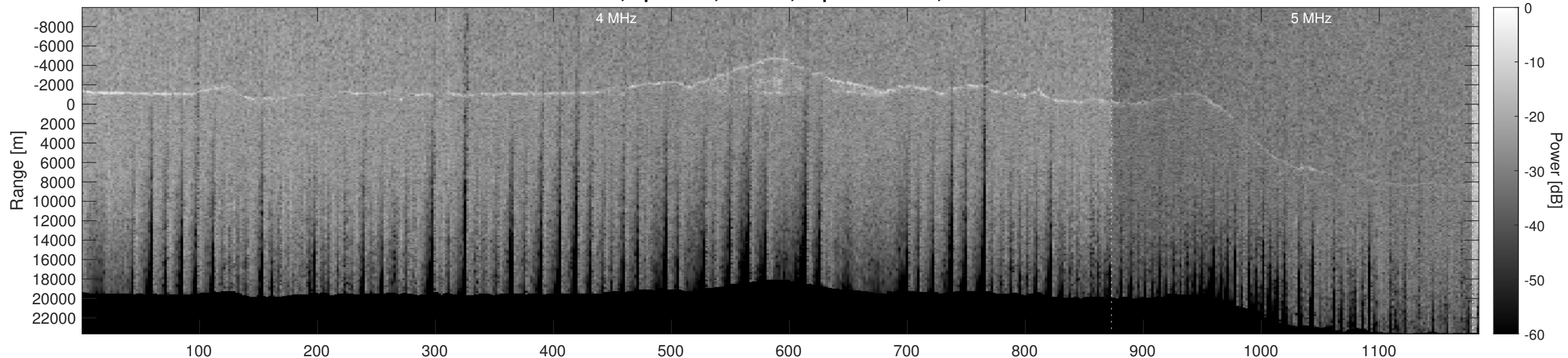
Orbit 12926, Optimized, Window, Depth-Corrected, Channel 2
