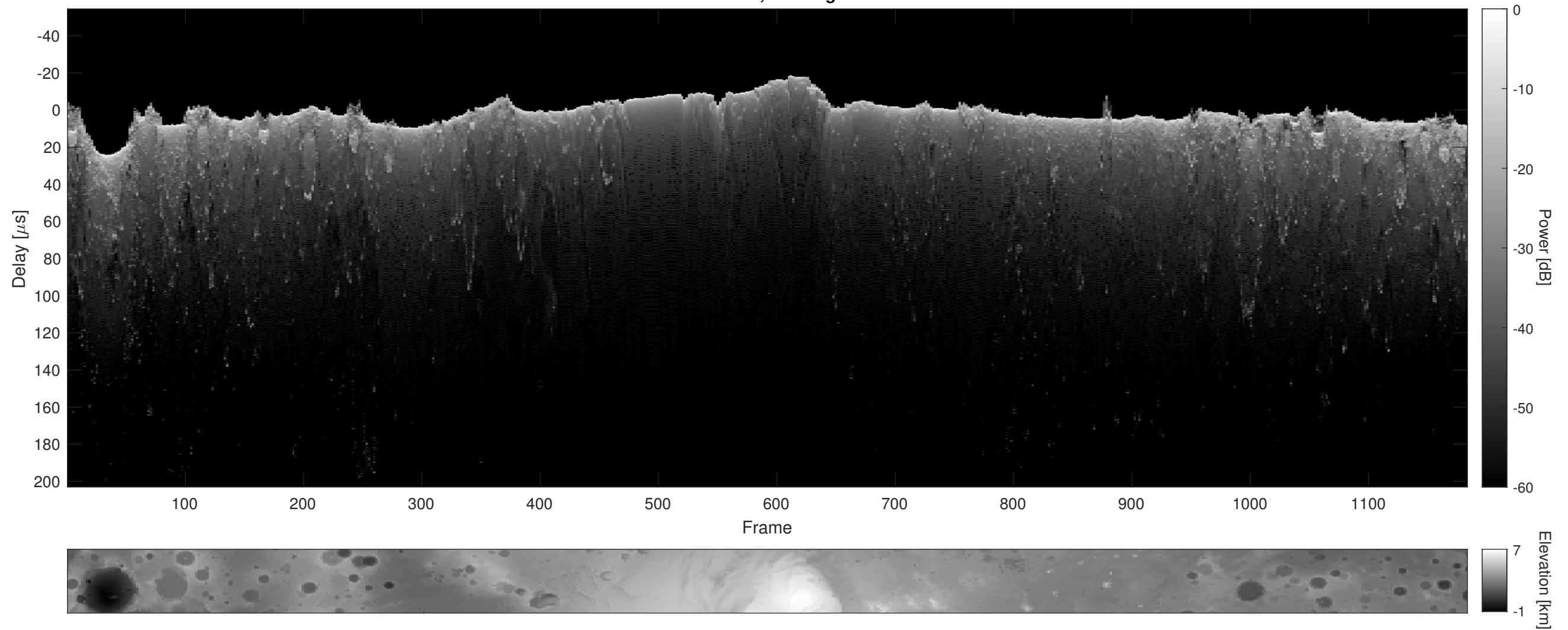
Orbit 12930, Cluttergram
