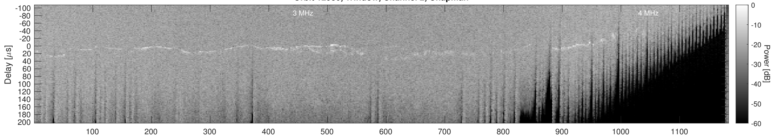
Orbit 12930, Window, Channel 2, Optimized
