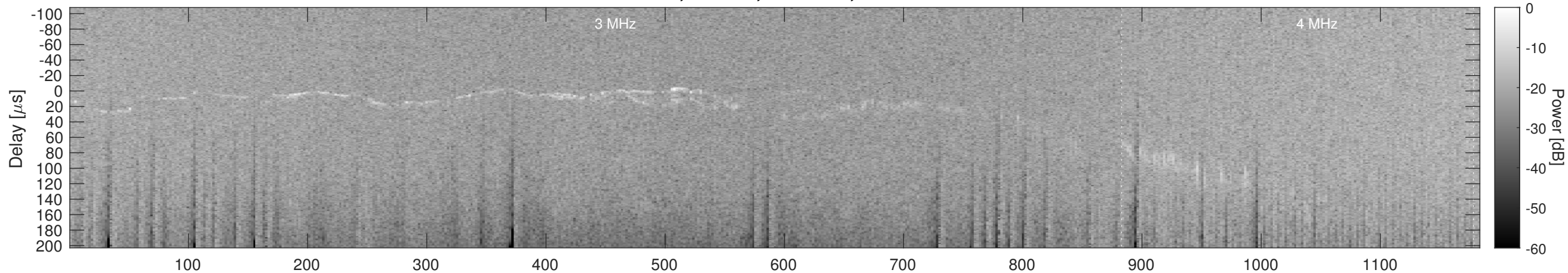
Orbit 12930, Window, Channel 2, Chapman
