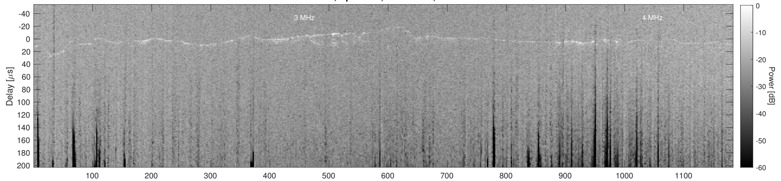
Orbit 12930, Cluttergram
