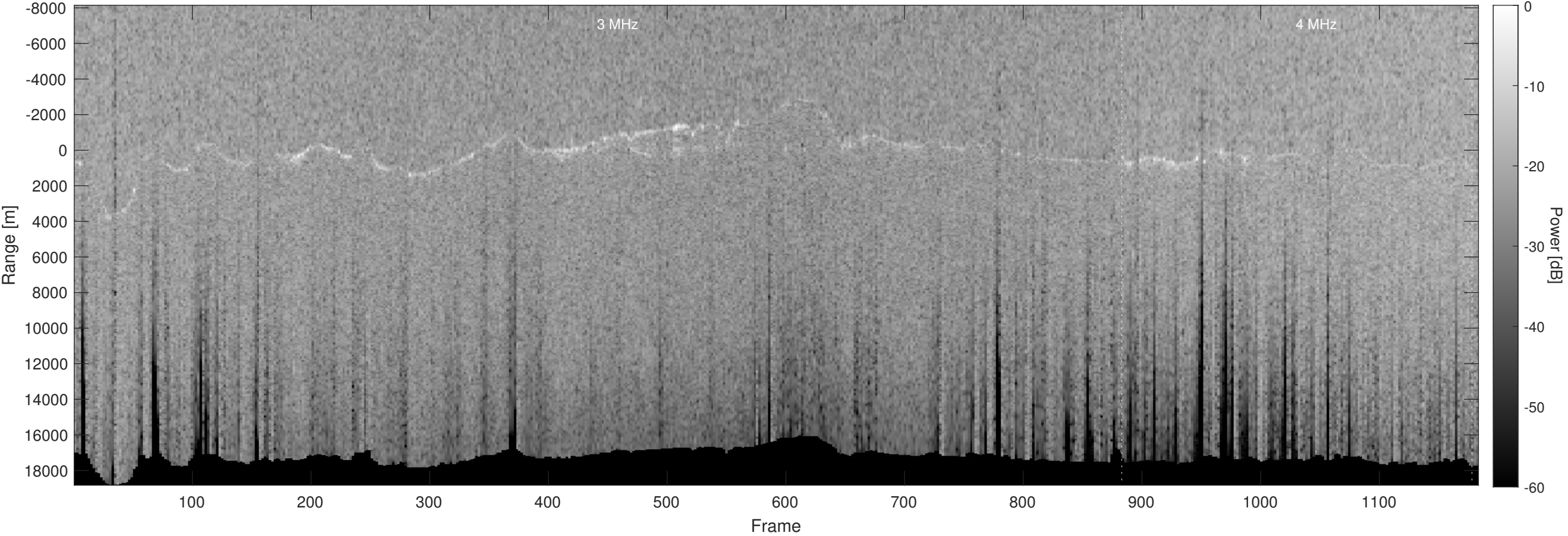
Orbit 12930, Optimized, Window, Depth-Corrected, Channel 2
