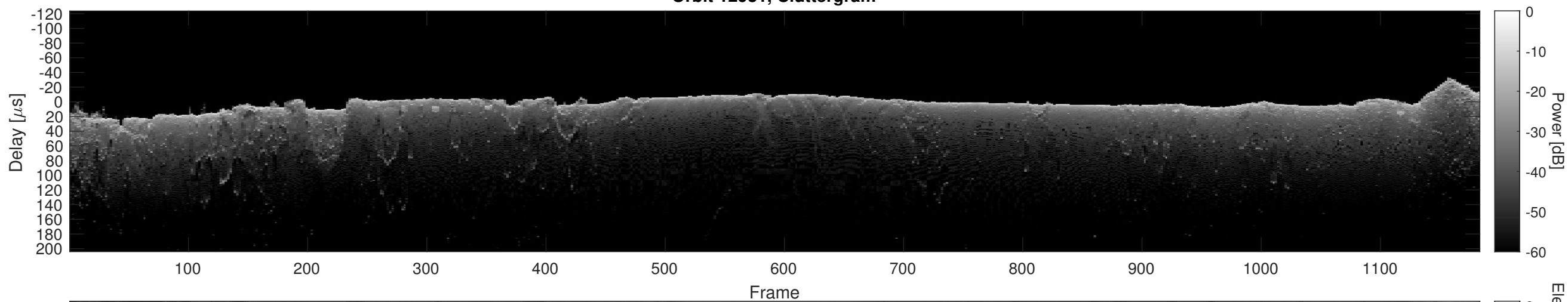
Orbit 12931, Cluttergram
