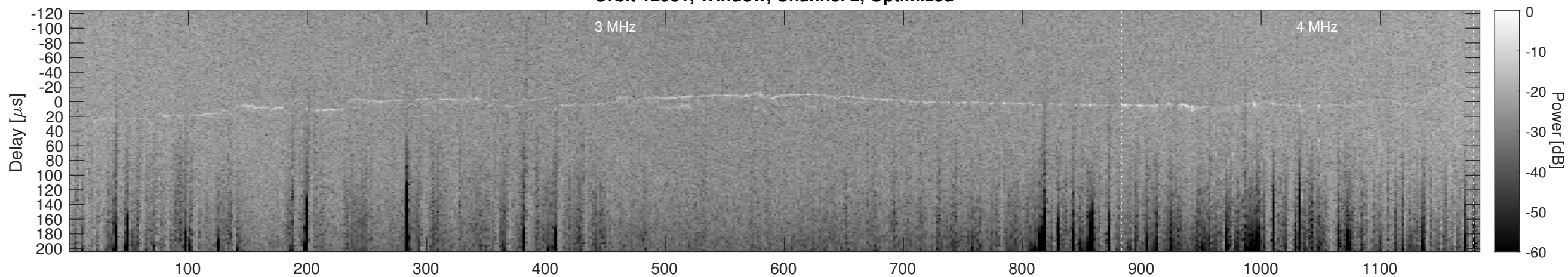
Orbit 12931, Cluttergram
