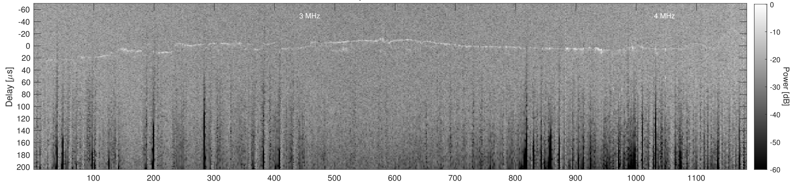
Orbit 12931, Cluttergram
