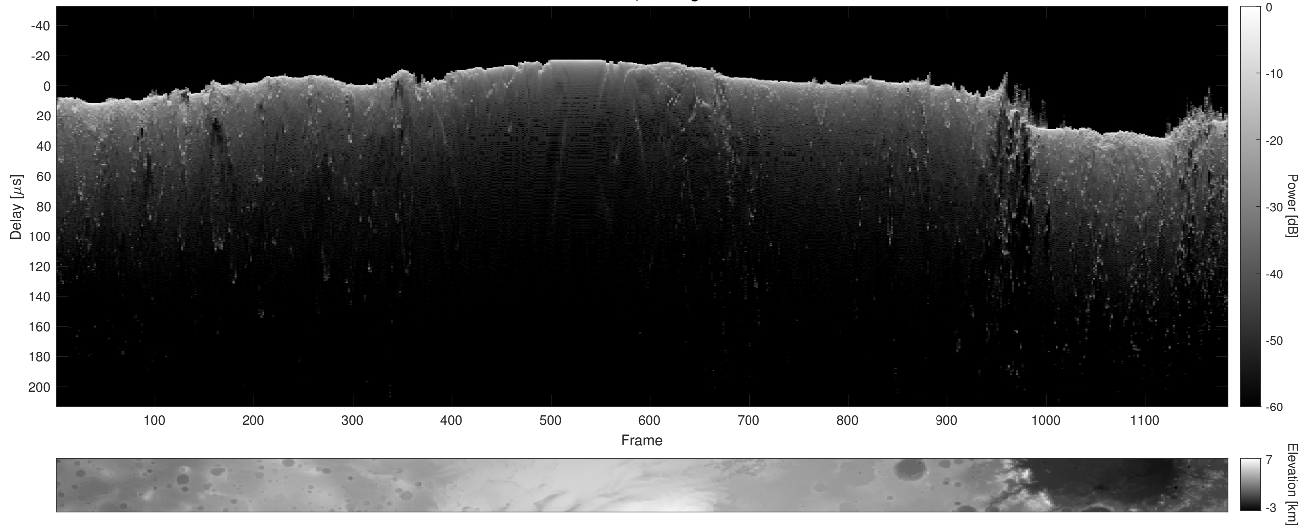
Orbit 12934, Cluttergram
