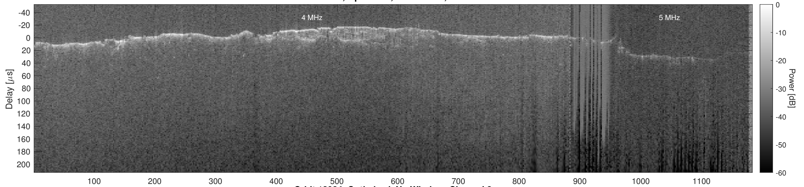
Orbit 12934, Optimized, No Window, Channel 2
