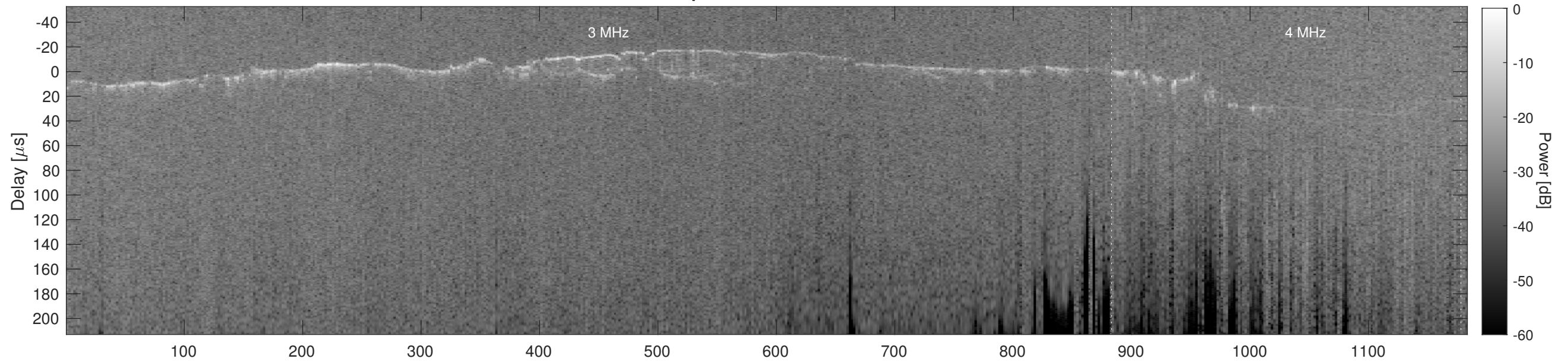
Orbit 12934, Cluttergram
