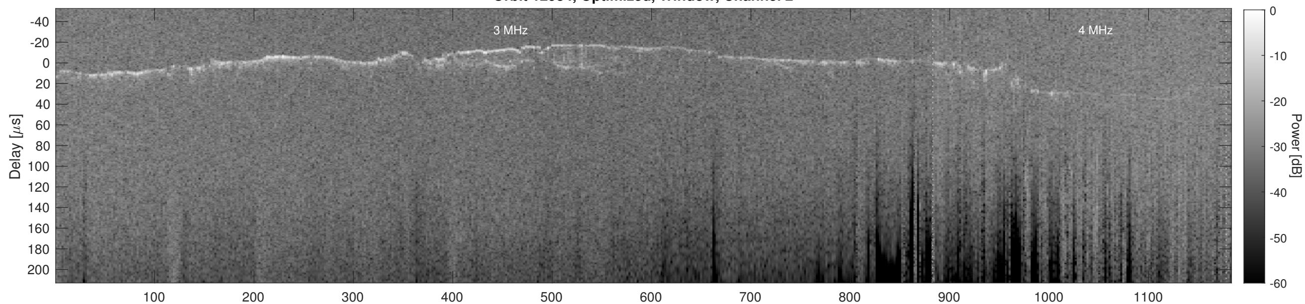
Orbit 12934, Cluttergram
