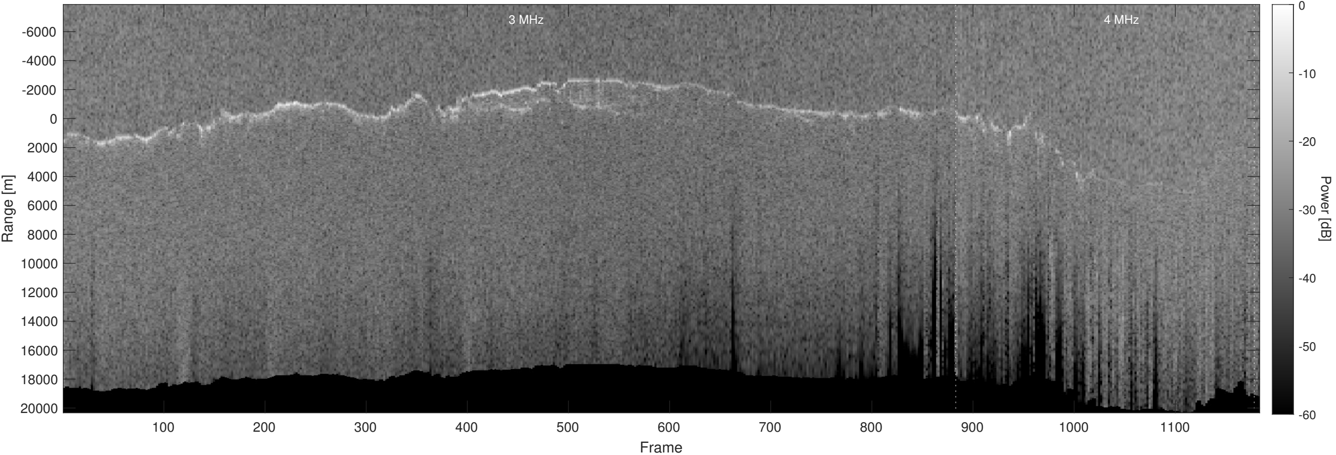
Orbit 12934, Optimized, Window, Depth-Corrected, Channel 2
