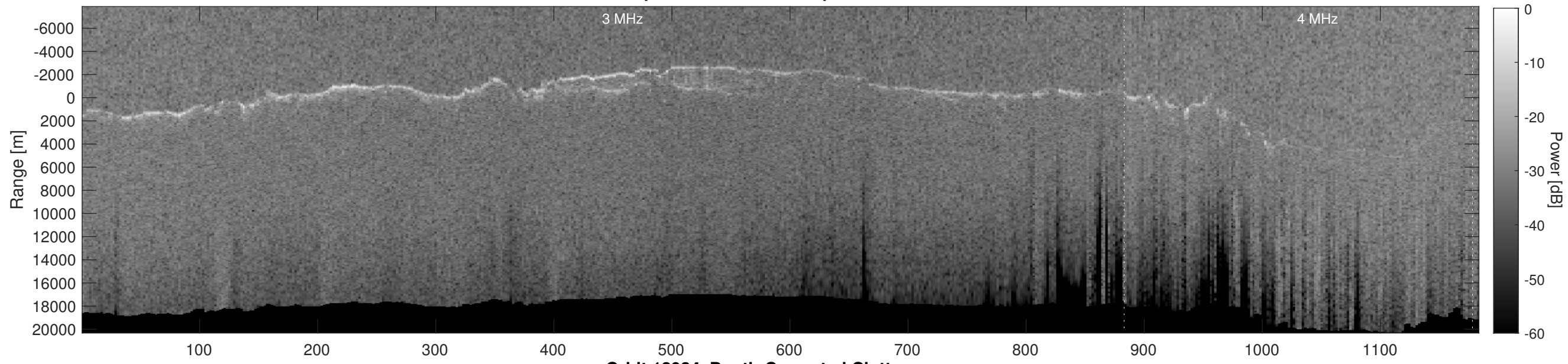
Orbit 12934, Depth-Corrected Cluttergram
