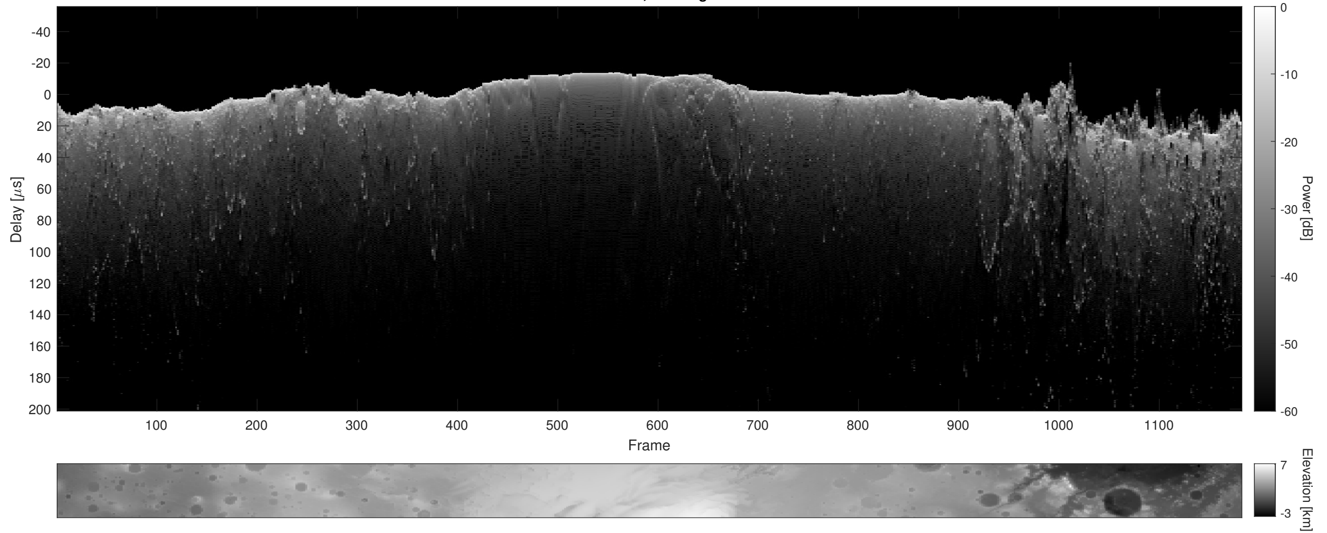
Orbit 12941, Cluttergram
