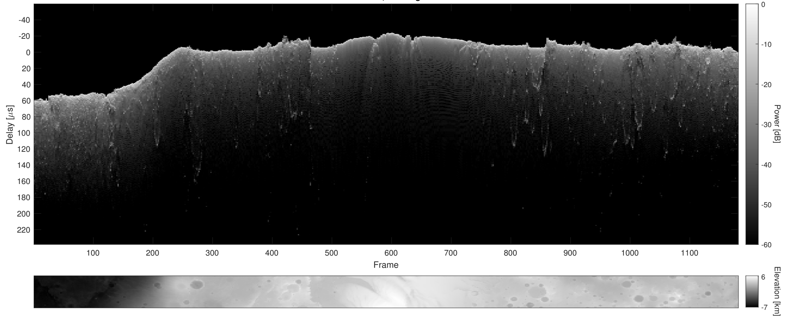
Orbit 12942, Cluttergram
