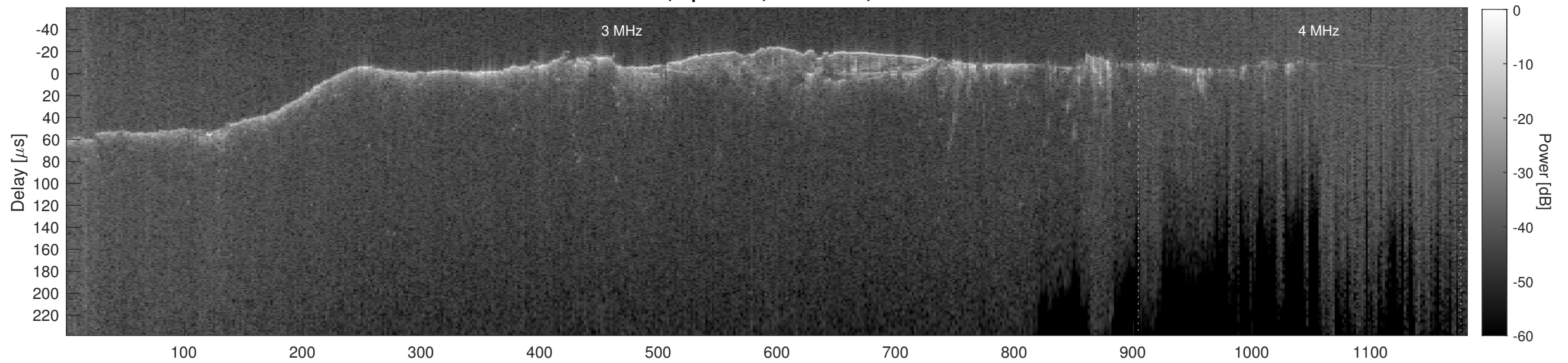
Orbit 12942, Cluttergram
