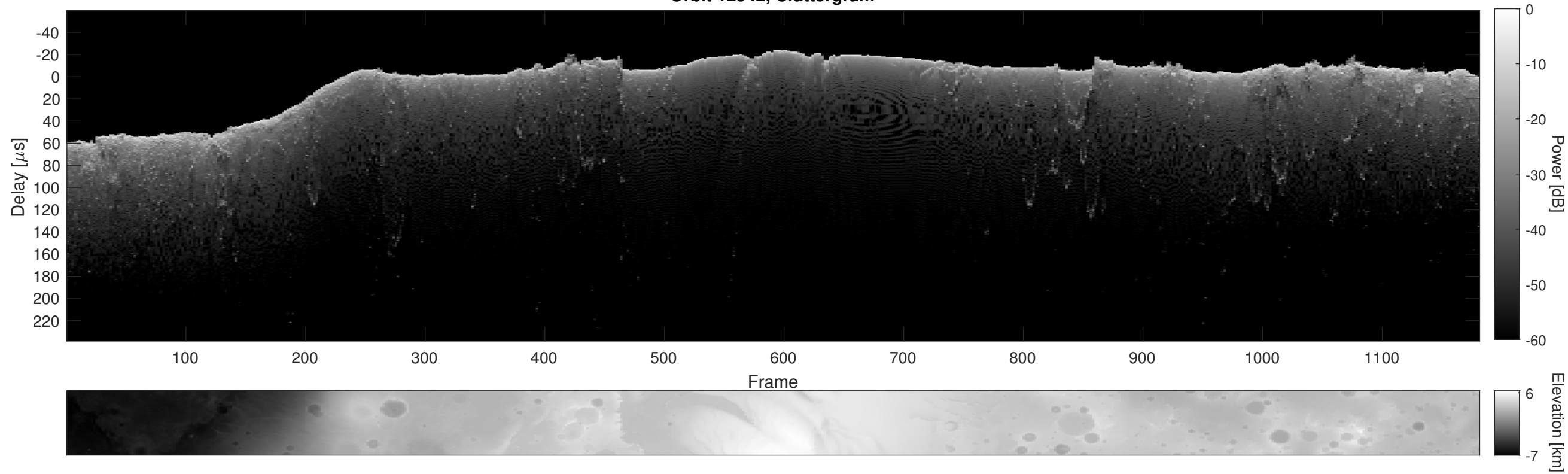
Orbit 12942, Cluttergram
