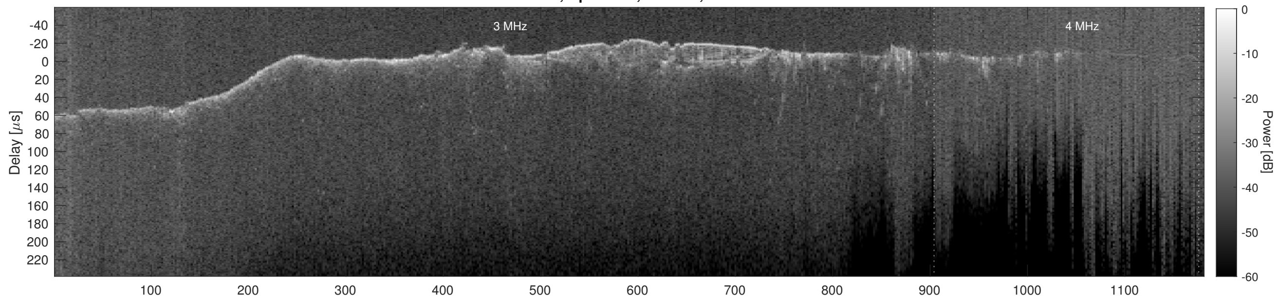
Orbit 12942, Cluttergram
