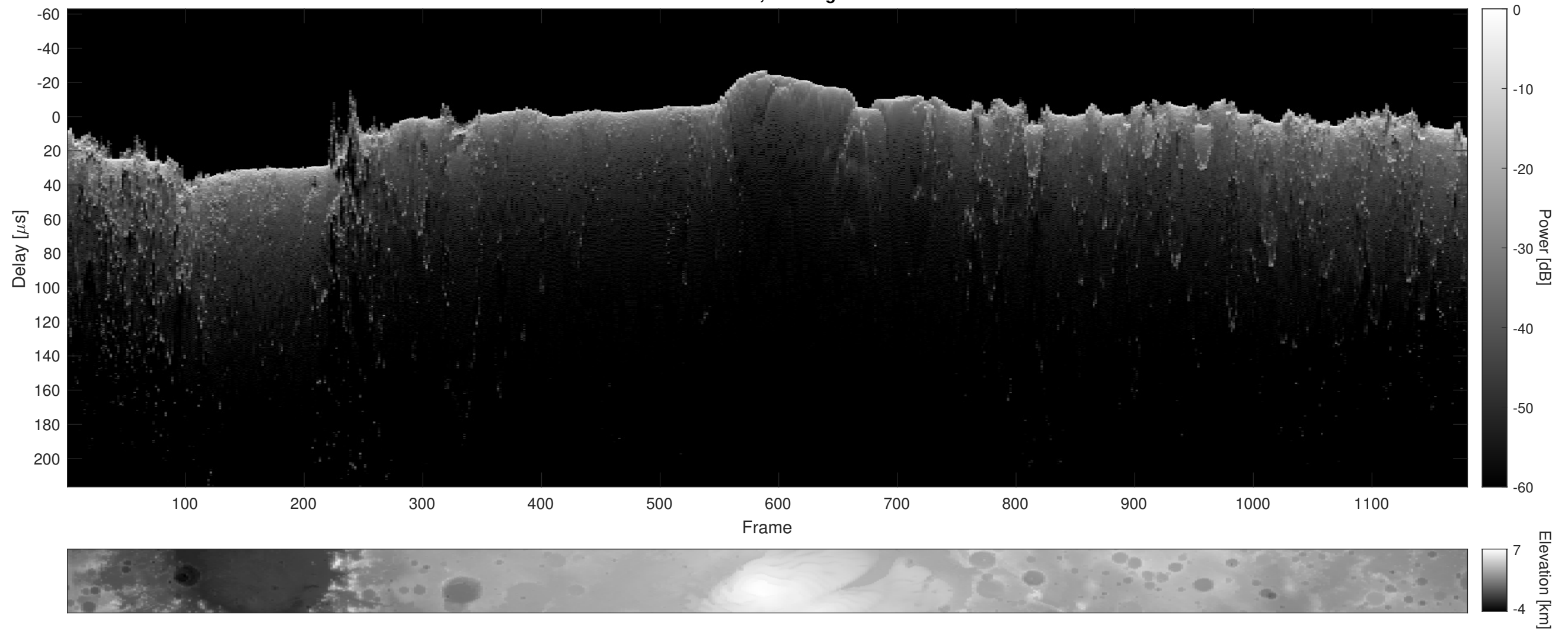
Orbit 12943, Cluttergram
