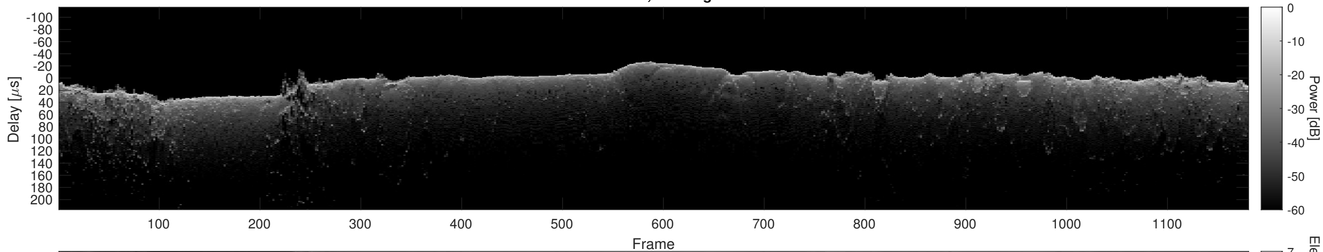
Orbit 12943, Cluttergram
