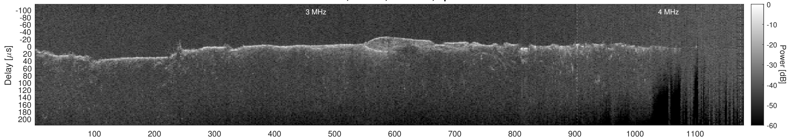
Orbit 12943, Cluttergram
