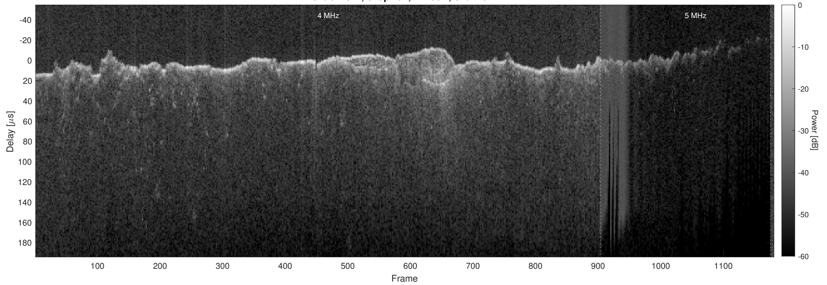
Orbit 12944, Chapman, Window, Channel 2
