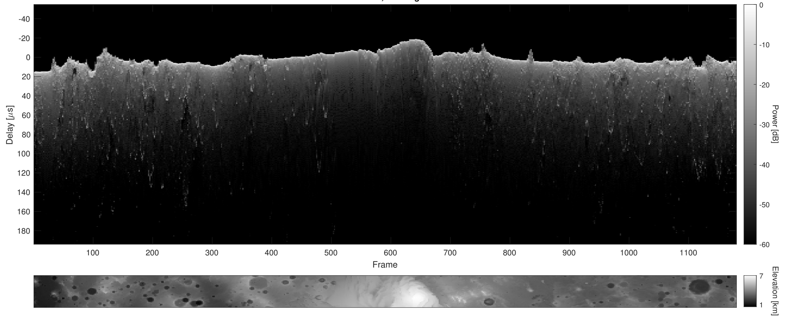
Orbit 12944, Cluttergram
