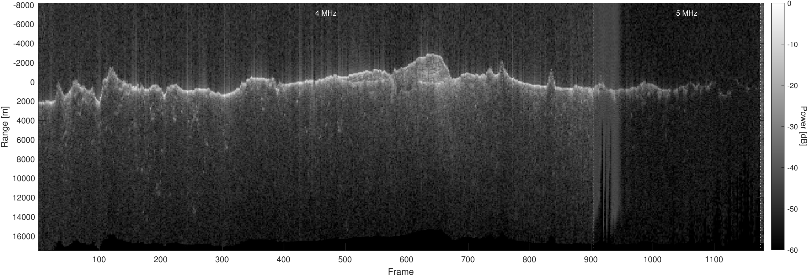
Orbit 12944, Optimized, No Window, Depth-Corrected, Channel 2
