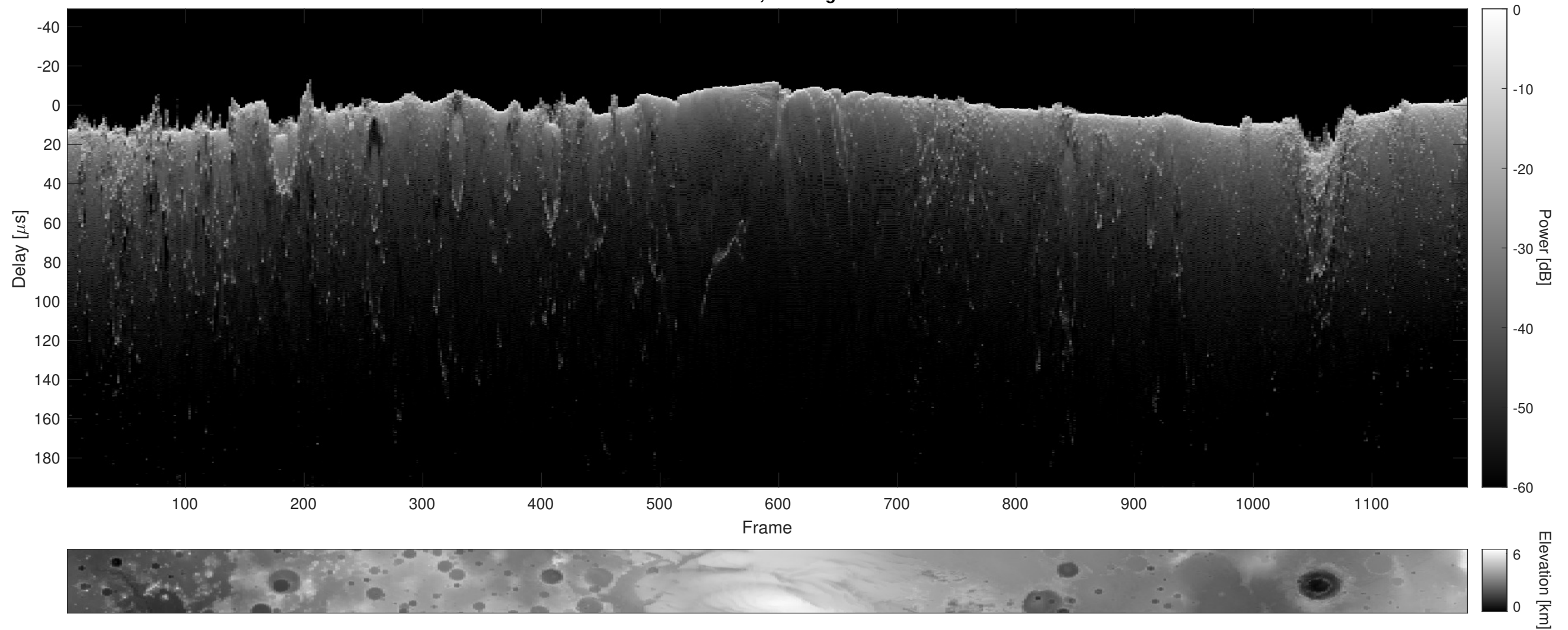
Orbit 12945, Cluttergram
