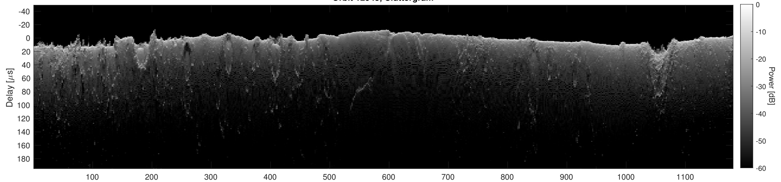
Orbit 12945, Cluttergram
