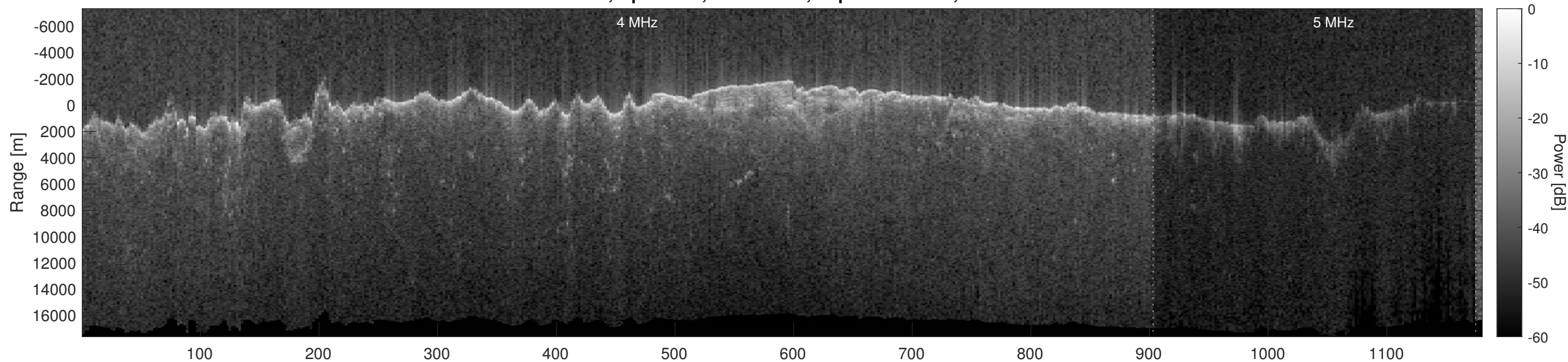
Orbit 12945, Optimized, No Window, Depth-Corrected, Channel 2
