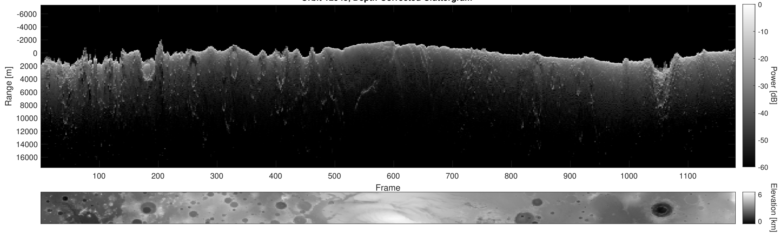
Orbit 12945, Depth-Corrected Cluttergram
