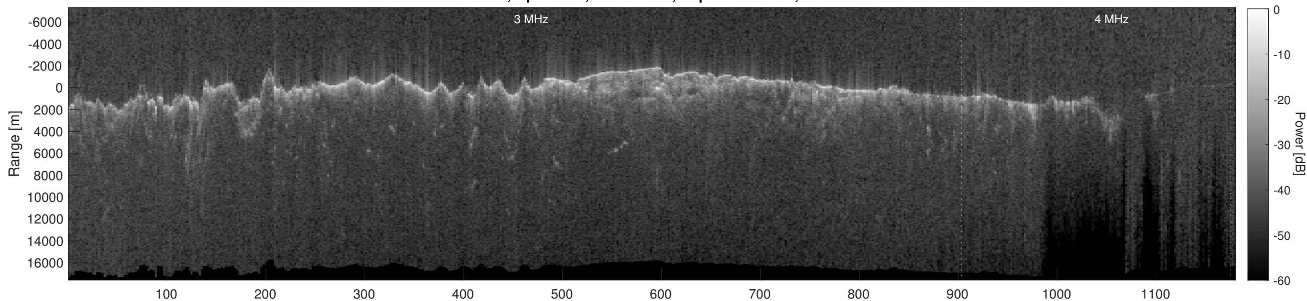
Orbit 12945, Depth-Corrected Cluttergram
