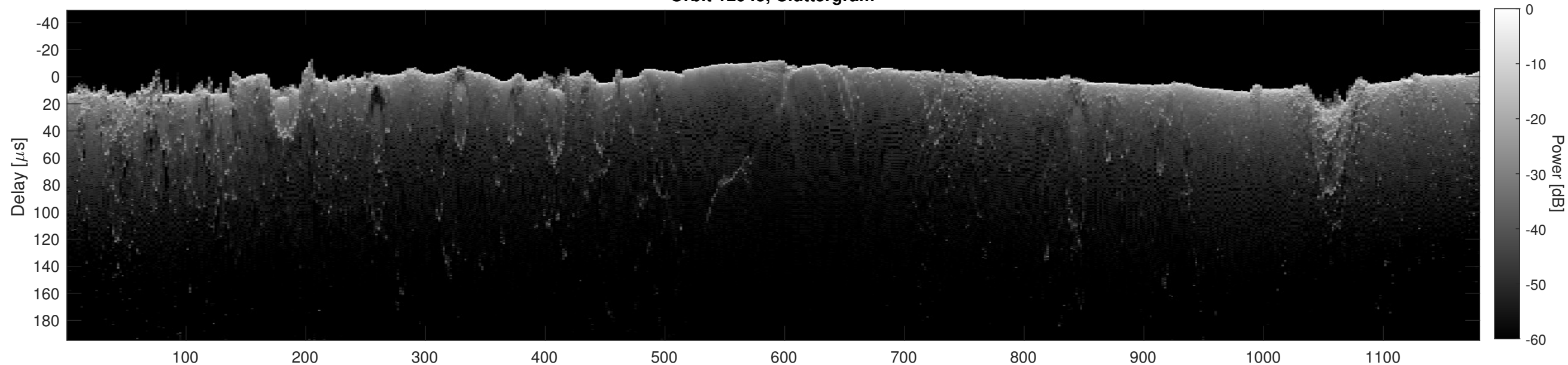
Orbit 12945, Cluttergram
