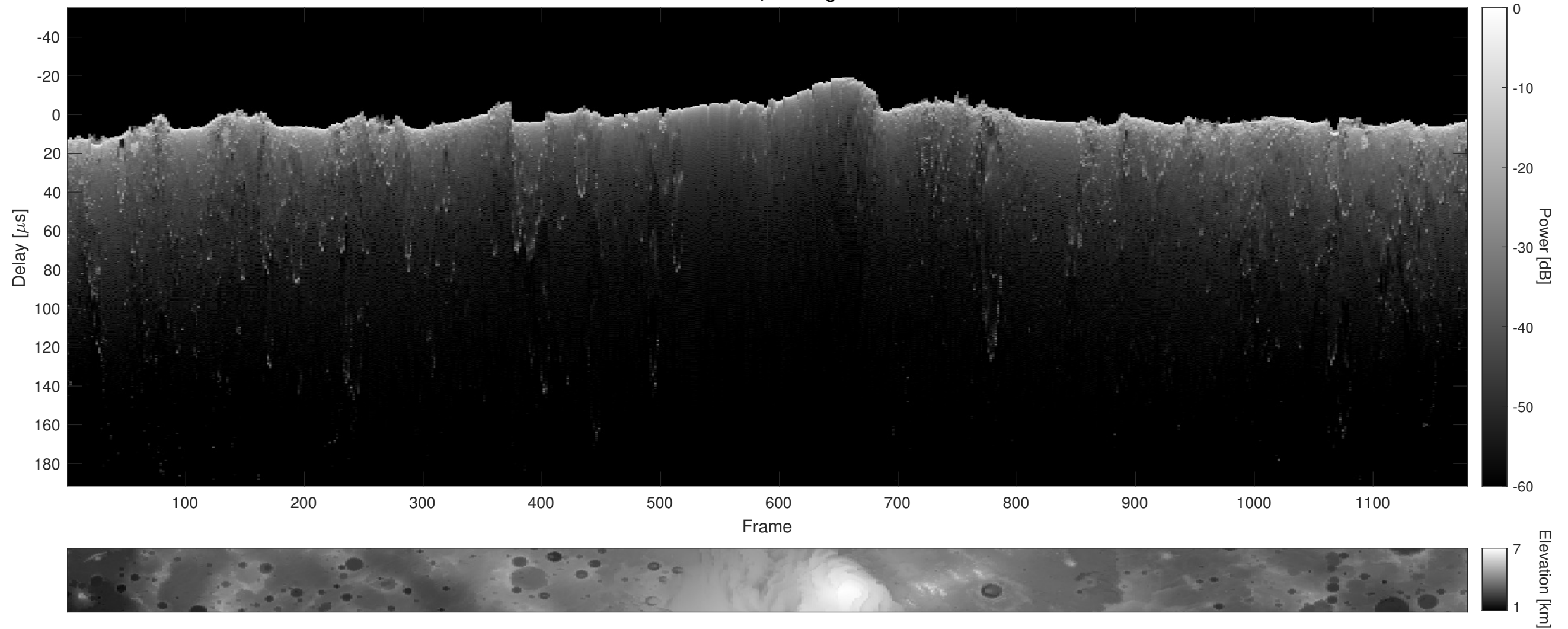
Orbit 12951, Cluttergram
