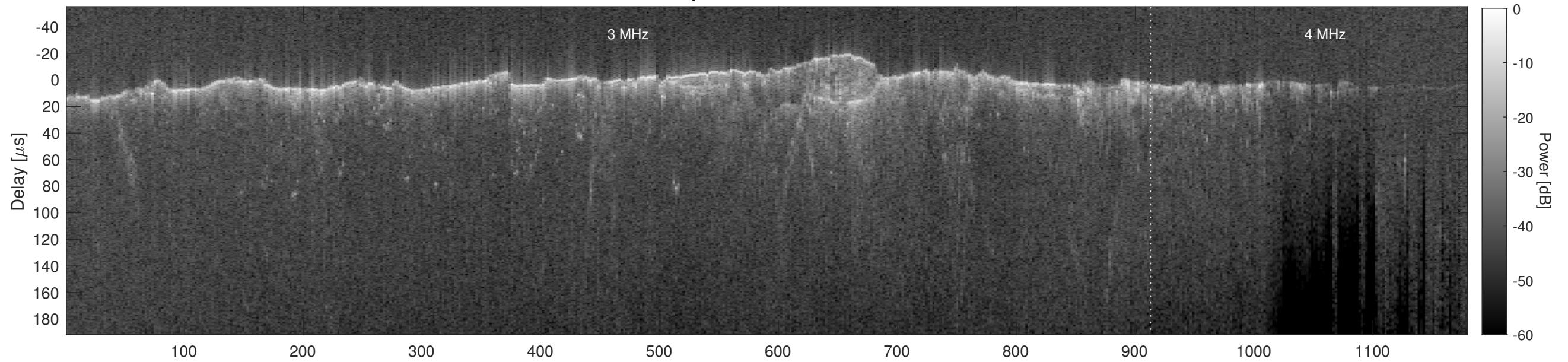
Orbit 12951, Cluttergram
